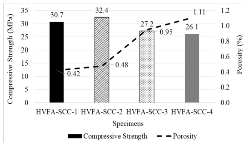
Figure 2. Correlation between compressive strength and porosity
