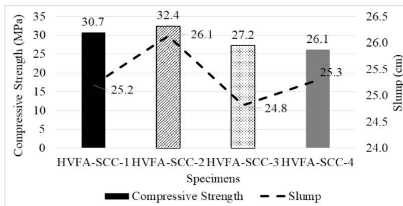
Figure 4. Correlation between compressive strength and slump
