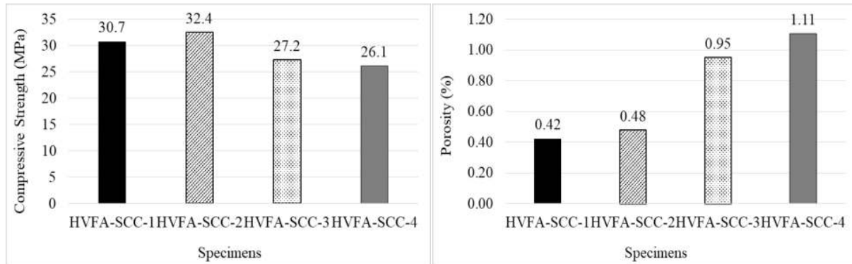
Figure 1. Compressive strength and porosity of HVFA-SCC specimens
