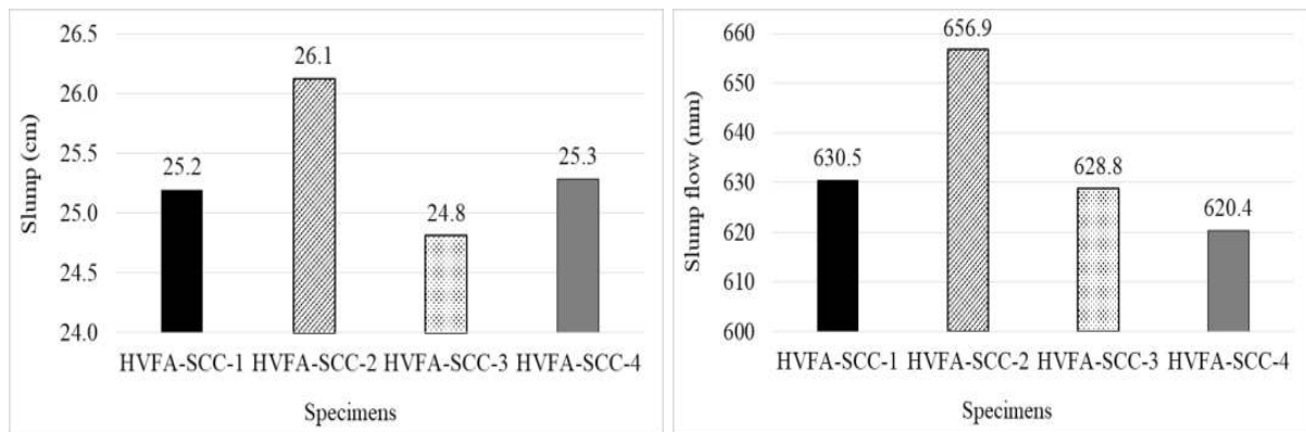
Figure 3. Slump and slump flow of HVFA-SCC specimens
