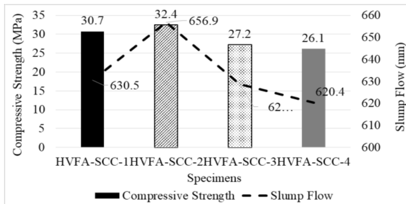
Figure 5. Correlation between compressive strength and slump flow
